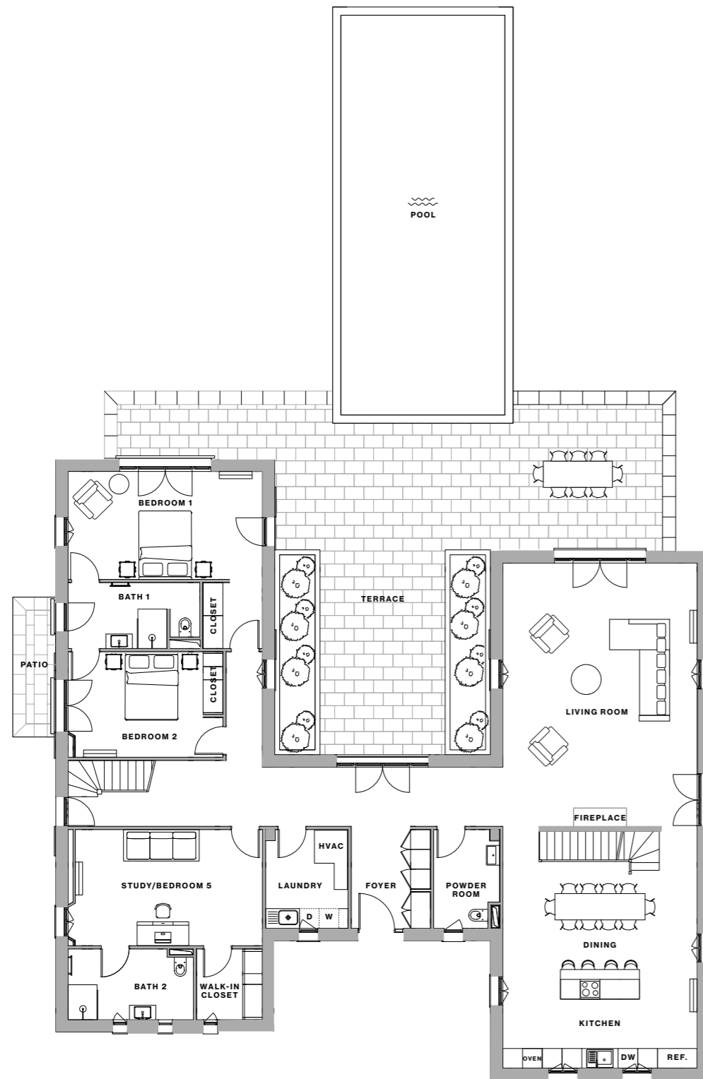
GROUND FLOOR
