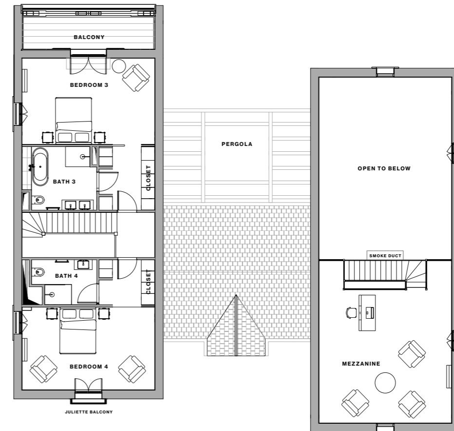
FIRST FLOOR
